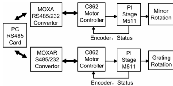
Fig.1 Wiring diagram of hardware.
