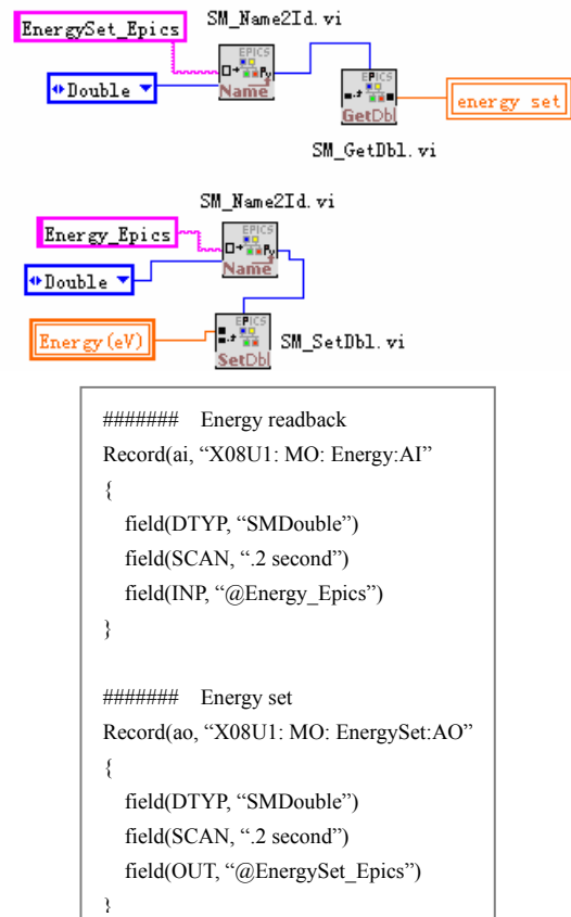
Fig.3 Data interface between LabVIEW and EPICS.
