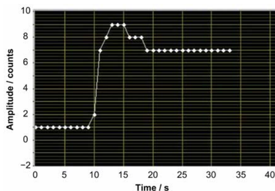
Fig.5 Test of dynamic step response.
